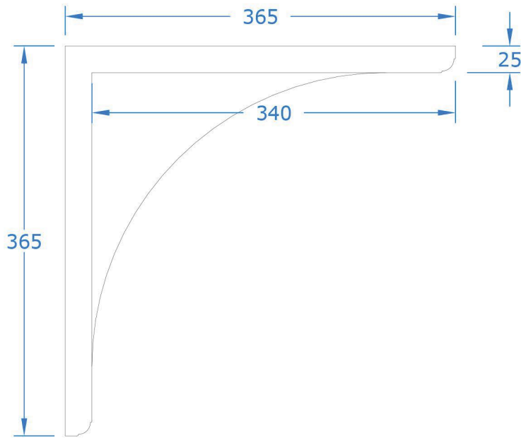
Side Elevation
